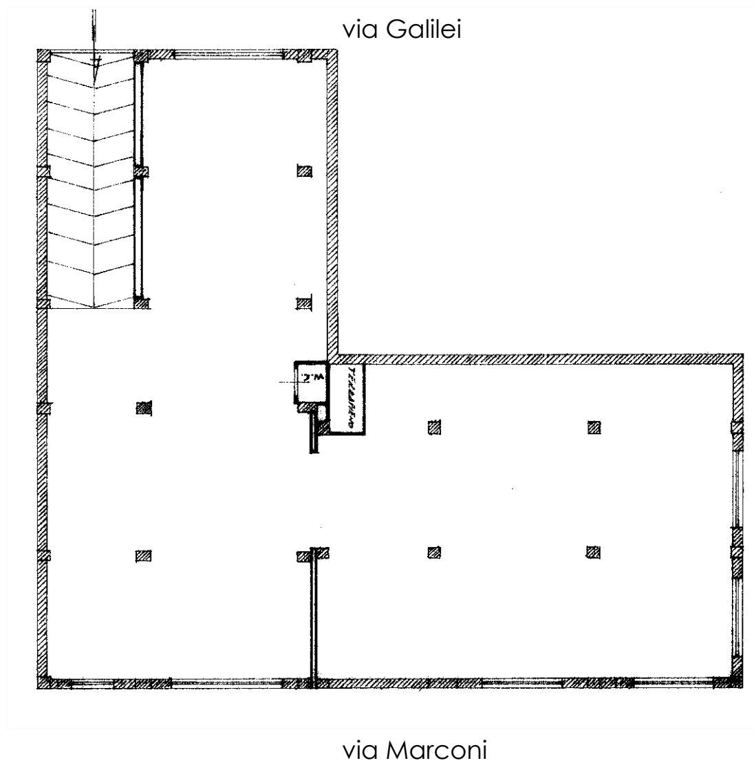
PIANO INTERRATO_ scala 1:200 Locale deposito Hint. = 2,80m NCEU: FG. 23 P.LLA 163 SUB 15 Sup. = mq. 406,00
